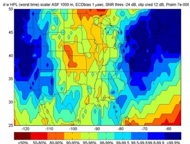
Figure 10. Expected Enroute (RNP 1.0) Availability worst case time of year [18]
